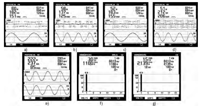
FIGURE 19. Experimental results for a RL load ( R = 430 \Omega , L = 200 mH). Voltage and power per stage: a) w = 6 , b) w = 7 , c) w = 8 , d) w = 9 ; e) output voltage and power; THD: f) output voltage; g) output current.
