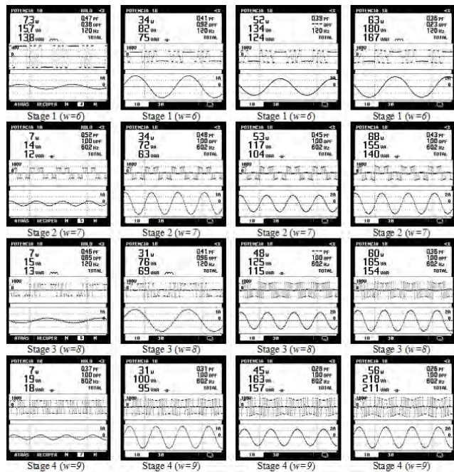
FIGURE 18. Power equalization measurements for resistive loads: a) 430 \Omega resistive load (28.3 W); b) 90 \Omega resistive load (130 W); c) 61 \Omega resistive load (198 W); d) 48 \Omega resistive load (247 W).
