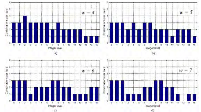
FIGURE 9. Distribution histograms of redundancy vs. levels: a) 4:5:6:7 ratio; b) 5:6:7:8 ratio; c) 6:7:8:9 ratio; d) 7:8:9:10 ratio.
