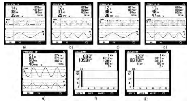
FIGURE 20. Experimental results for a RC load ( R = 430 \Omega , C = 24 \mu F ). Voltage and power per stage: a) w = 6 , b) w = 7 , c) w = 8 , d) w = 9 ; e) output voltage and power; THD: f) output voltage; g) output current.
