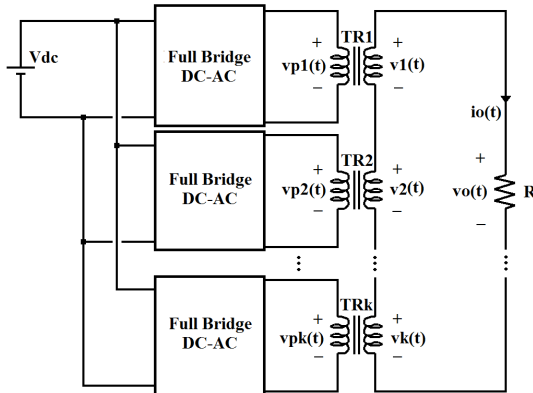
FIGURE 1. Transformer-based cascaded multilevel inverter.
