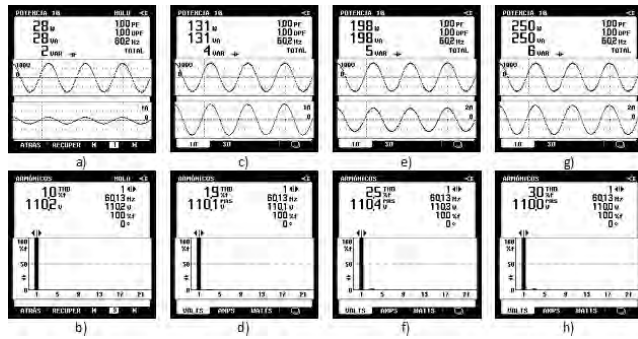
FIGURE 17. Voltage quality measurements for resistive loads. 430 \Omega : a) output power b) THD; 90 \Omega : c) output power d) output voltage THD; 61 \Omega : e) output power f) THD; 48 \Omega : g) output power h) THD.
